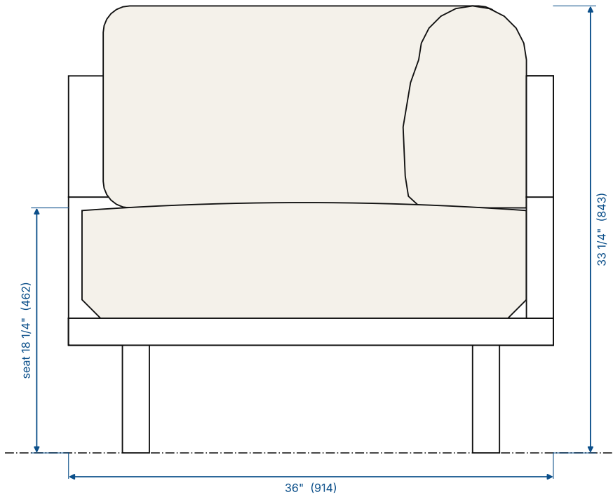
FRONT ELEVATION 1:10
