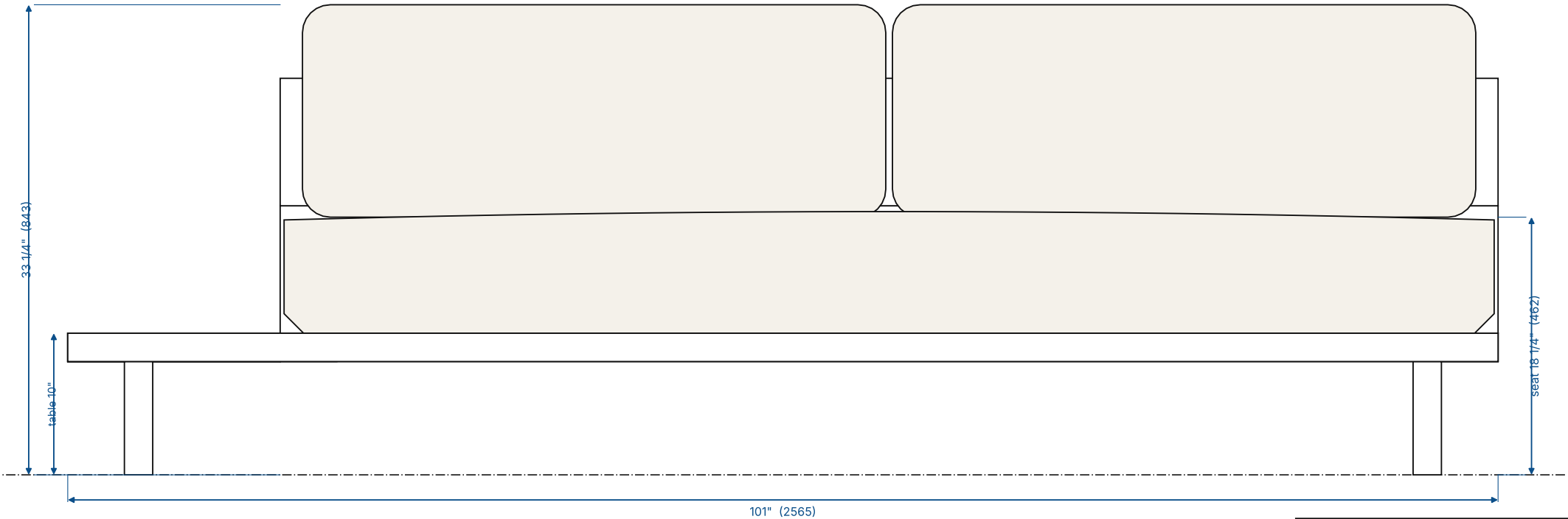
FRONT ELEVATION 1:10
